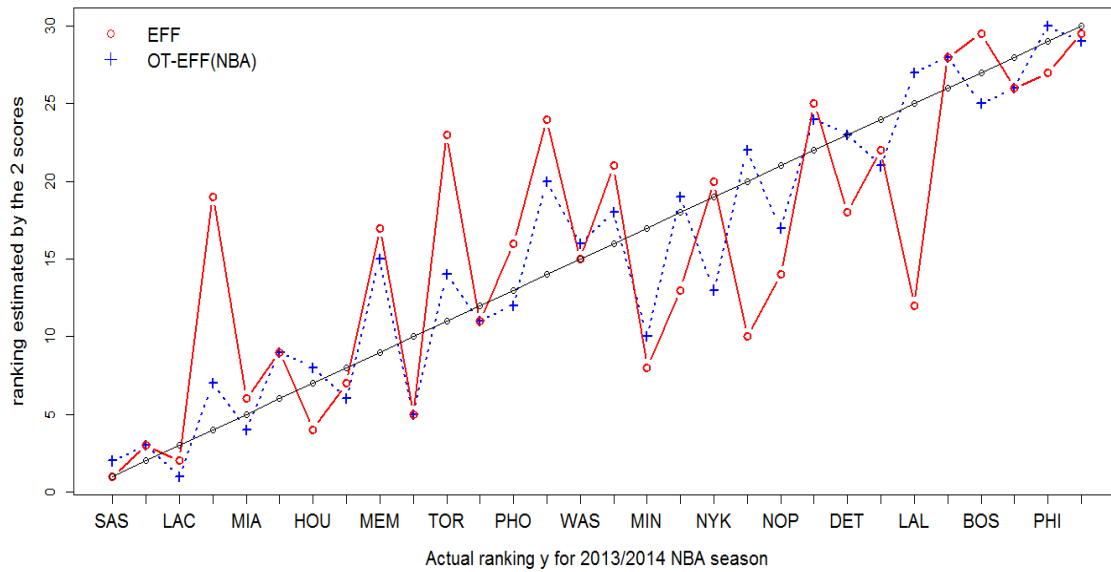
FIGURE 9. The estimated ranking for the NBA data set of 2013/2014: EFF is in red, OT-EFF in blue.
