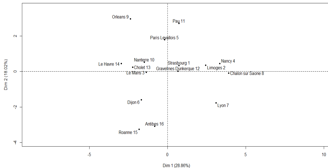
FIGURE 10. Principal Component Analysis (PCA) of the 2014 PRO A season (graph of individuals).
