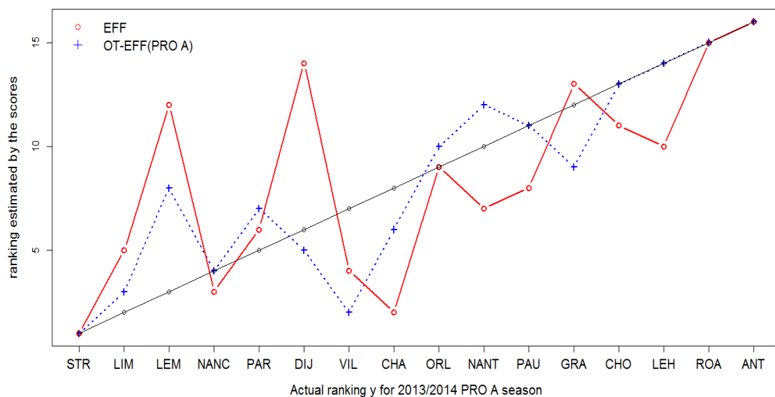
FIGURE 8. The estimated ranking for the PRO A data set of 2013/2014: EFF is in red, OT-EFF in blue.
